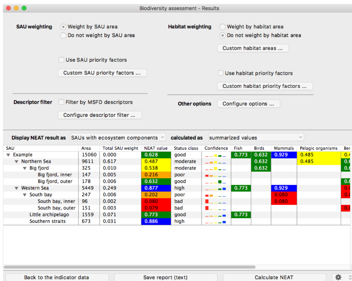
Figure 14. Window containing the results of an assessment.
