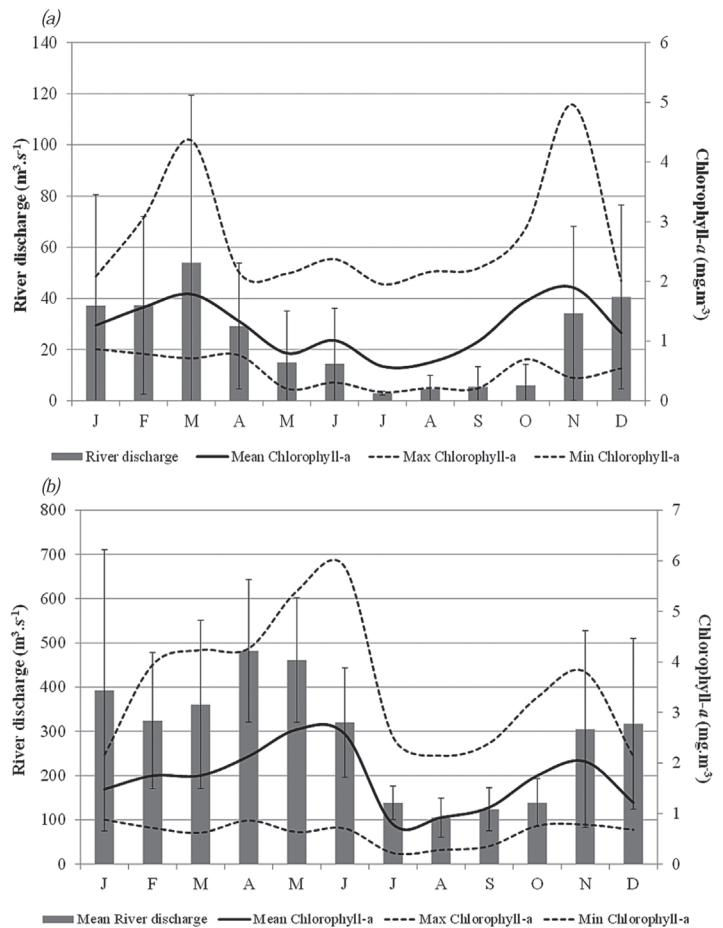
Figure 9. Monthly mean, maximum and minimum chl- a concentrations, and monthly mean river discharge and standard deviations, at the Nervión (a) and Adour (b) rivers, for the 2005-2010 period.
