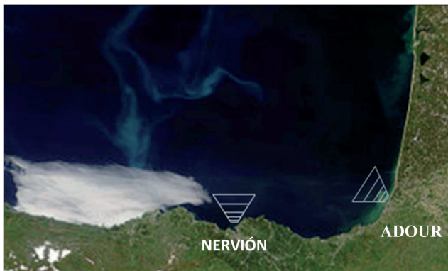
Figure 2. Polygons used to extract mean chl- a concentrations at different distances from the river Nervión and Adour mouths (MODIS Terra, 17/05/2004).
