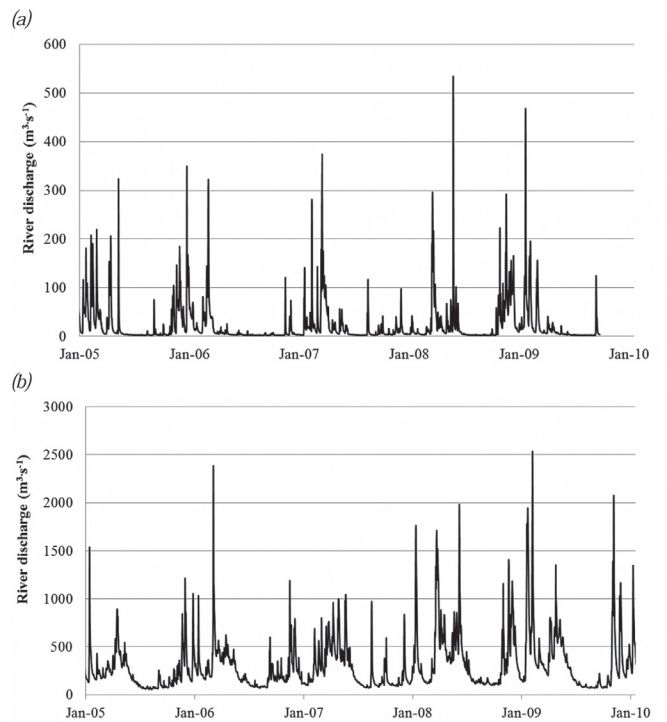
Figure 12. Time series of daily river discharges at the Nervión (a) and the Adour (b) river stations.
