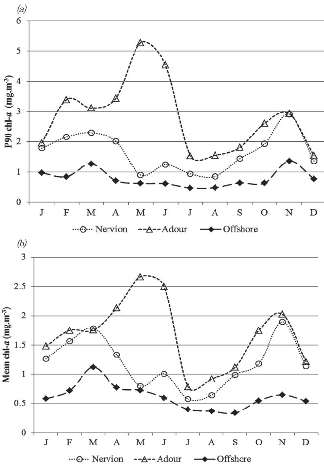
Figure 8. P90 Chl- a monthly values (a) and means (b) for the 2005-2010 period at 3 different locations: The Nervión river plume, the Adour river plume and the offshore reference station.
