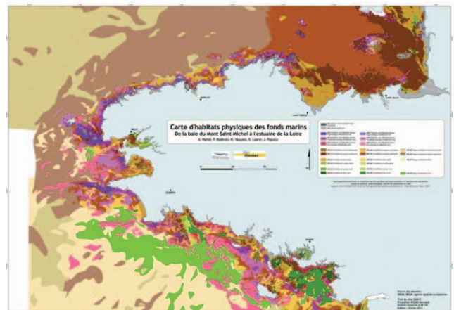
Figure 2. EUNIS physical habitats in Brittany.
