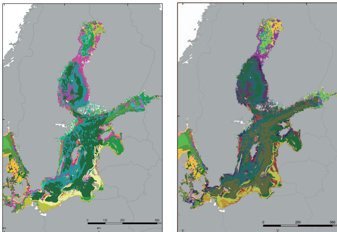
Figure 3. EUSeaMap for the Baltic Sea, with respectively 31 and 52 habitats depending on whether energy (3 classes) or salinity (4 classes) were introduced into the model.
